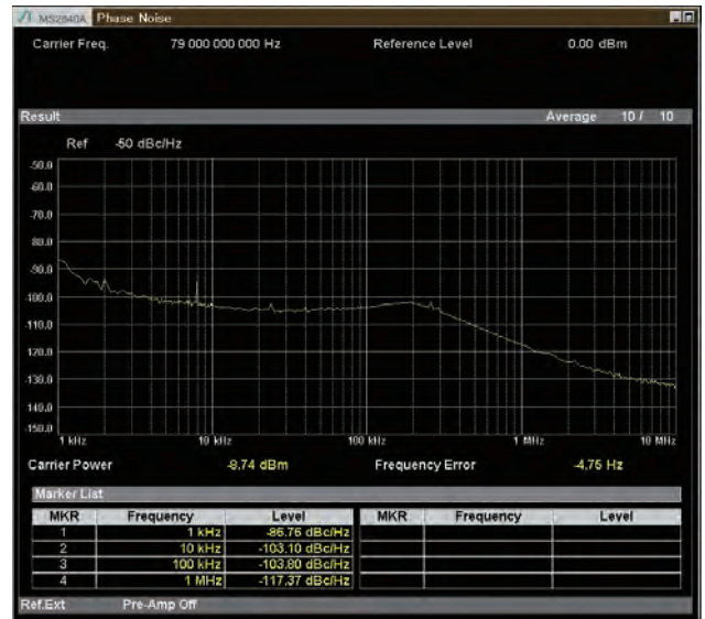
Phase Noise Measurement 79 GHz Measurement Frequency (Using High-Performance Waveguide Mixer MA2808A)
